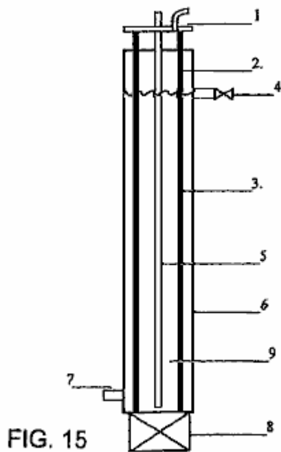
WIRES OR RODE IN TUBE REACTOR THE OUTER ELECTRODE SERVING AS BATH
